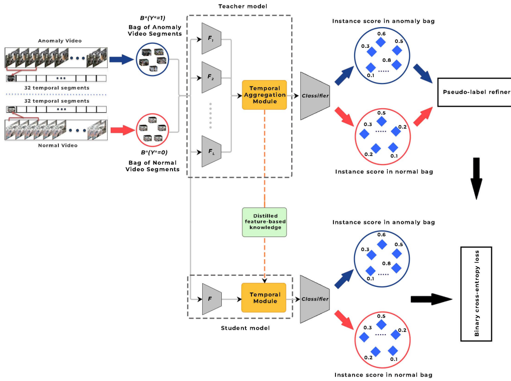
Figure 1: Student Model Training Pipeline
